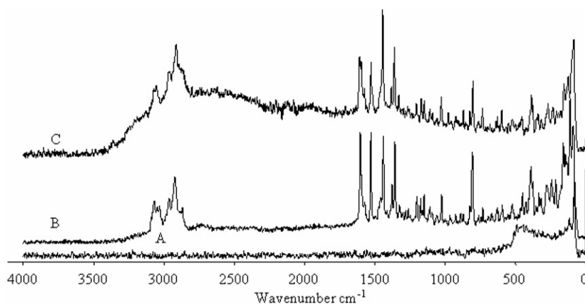
Fig. 5 Raman spectra of the pristine MCM-41 (A), the spacer modified homogeneous catalyst 3 (B) and the hybrid catalyst 4 (C).
