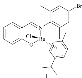
Fig. 1 Homogeneous catalyst 1 .
