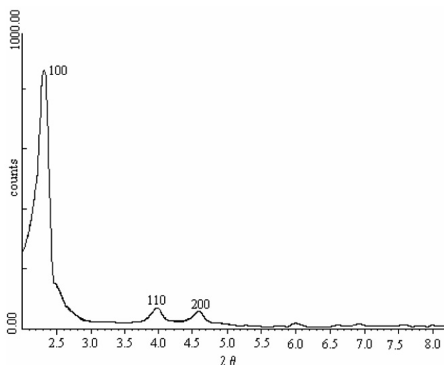
Fig. 3 XRD pattern of the pristine MCM-41.
