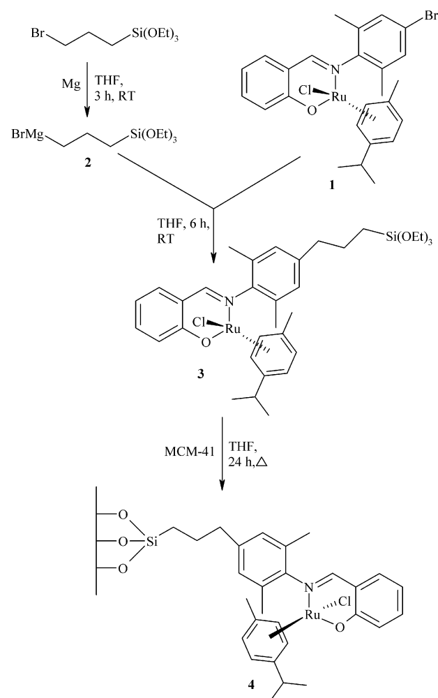
Scheme 2 Synthesis of the heterogeneous catalyst 4.
