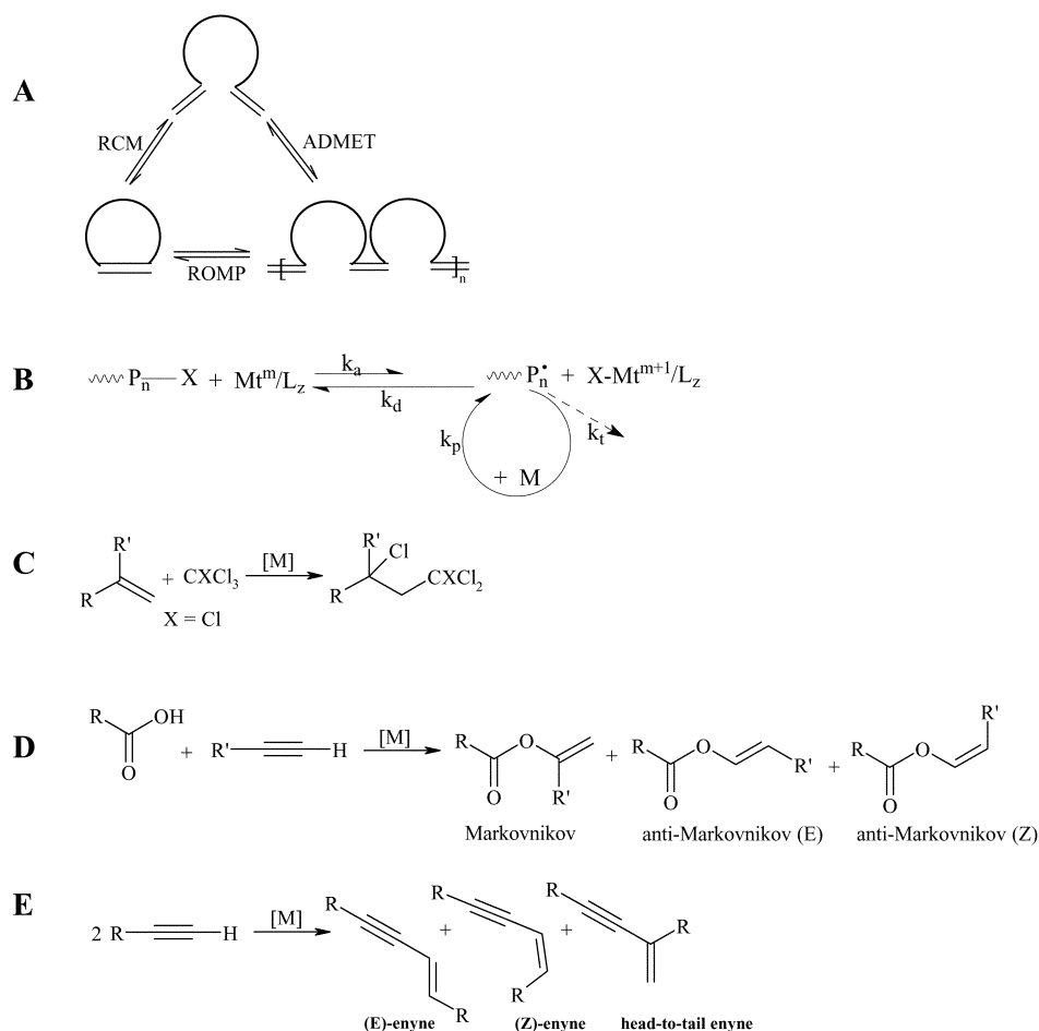
Scheme 1 Schematic representation of olefin metathesis (A), ATRP (B), Kharasch addition (C), vinylation (D) and dimerization (E).
