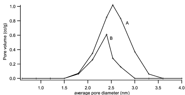
Fig. 4 Pore size distributions of both the pristine MCM-41 (A) and the heterogeneous catalyst 4 (B).
