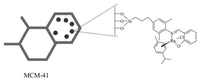
Fig. 2 Cartoon type representation of the hybrid catalytic system 4 .
